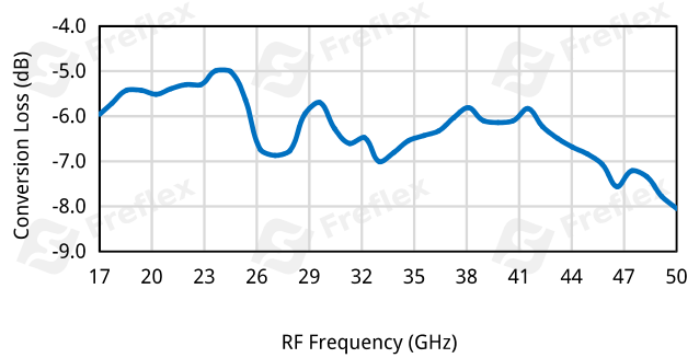
Downconversion Loss vs. Frequency @IF=100MHz @LO=15dBm
