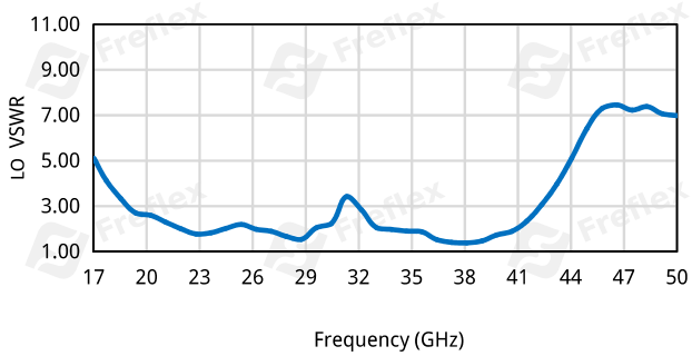
LO VSWR vs. Frequency @RF=33GHz @LO=14dBm
