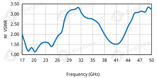
RF VSWR vs. Frequency @RF=33GHz @LO=14dBm
