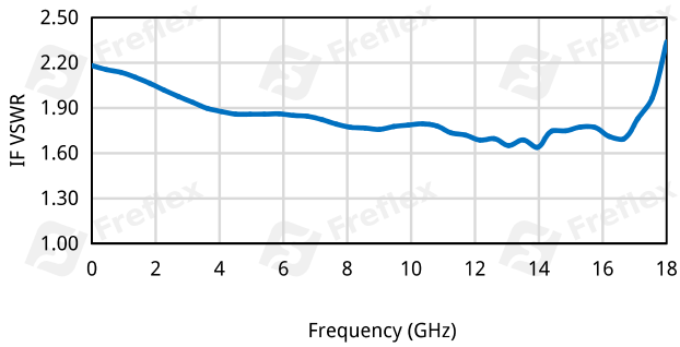
IF VSWR vs. Frequency @RF=33GHz @LO=15dBm
