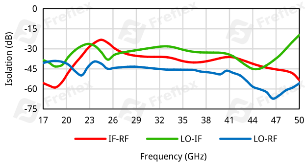
Isolation vs. Frequency @LO=0dBm
