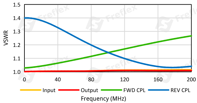
VSWR vs. Frequency
