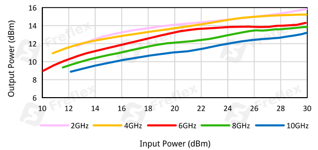
Output Power vs. Input Power vs. Frequency
