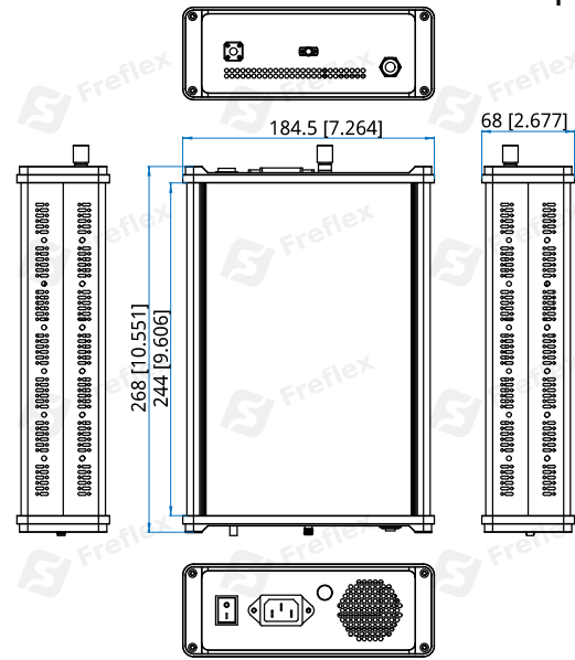
Outline E: Enclosure 0-000006
