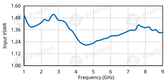
Input VSWR vs. Frequency
