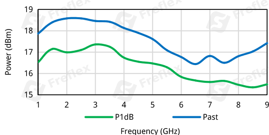
Power vs. Frequency
