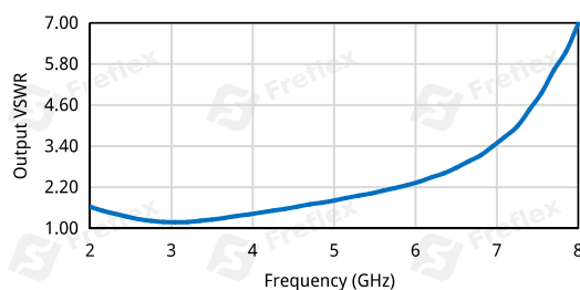
Output VSWR vs. Frequency
