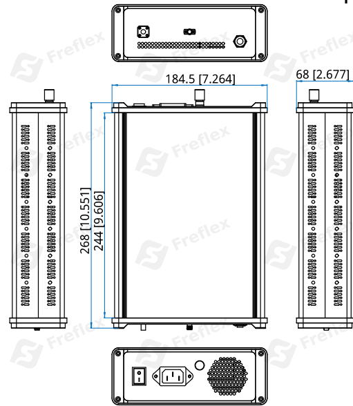
Outline E: Enclosure 0-000006
