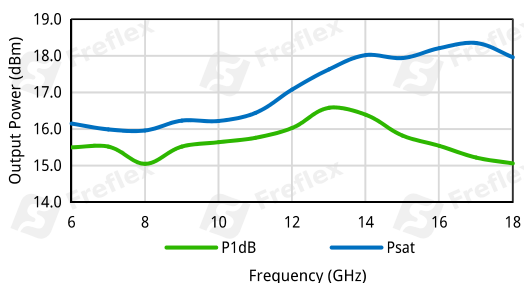
Output Power vs. Frequency
