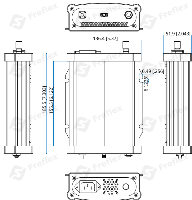
Outline C: Enclosure 0-000009-V2
