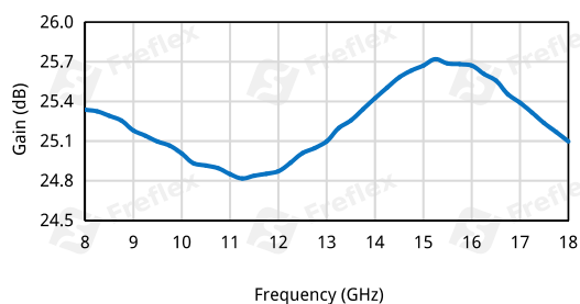
Gain vs. Frequency
