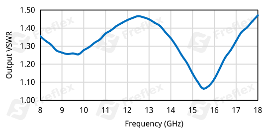
Output VSWR vs. Frequency
