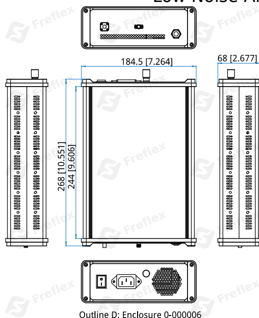
Outline D: Enclosure 0-000006
