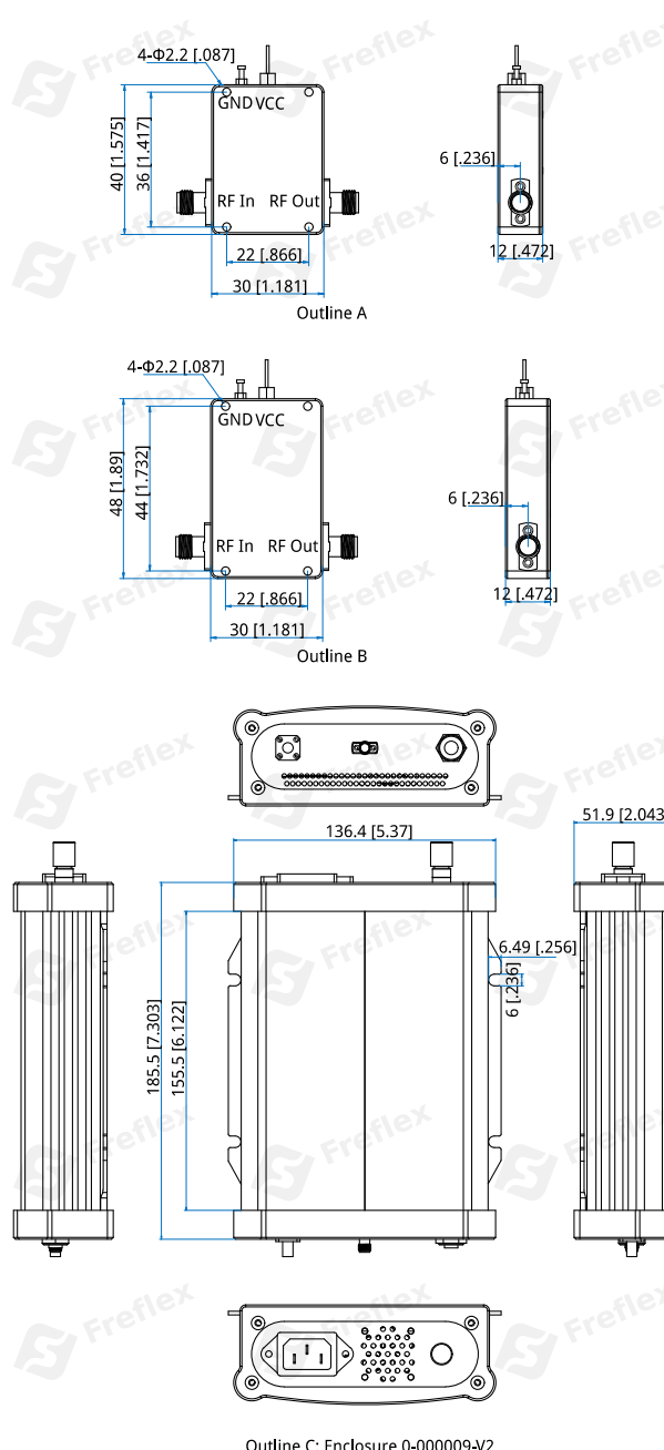
Outline C: Enclosure 0-000009-V2
