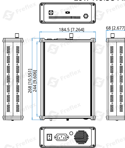
Outline D: Enclosure 0-000006
