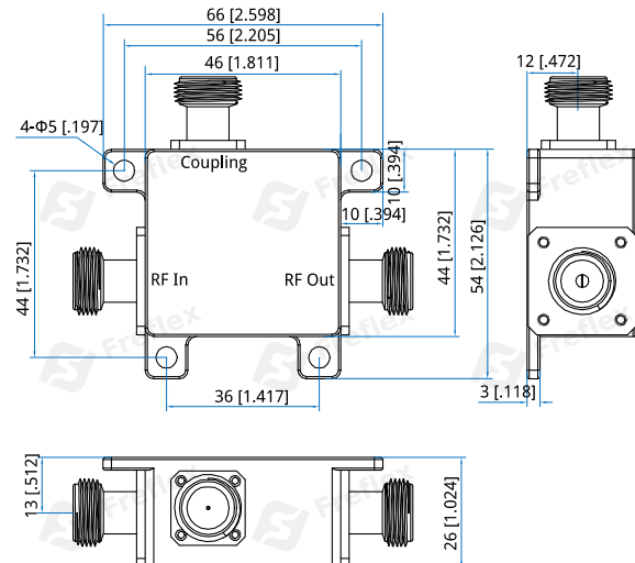
Outline B
