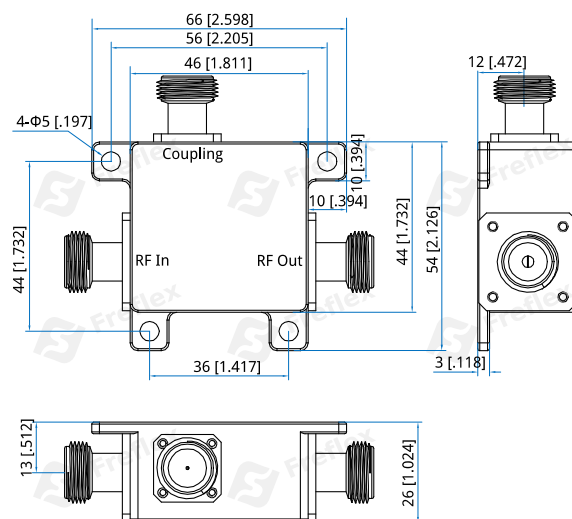
Outline B
