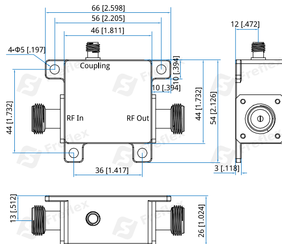
Outline A
